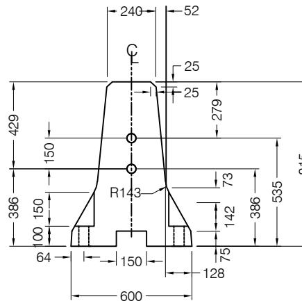
END VIEW DETAIL END A
