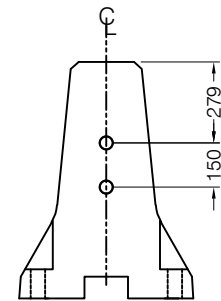
END VIEW DETAIL END B
