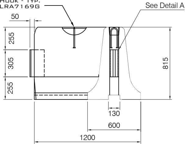
END VIEW DETAIL FEMALE CONNECTOR
