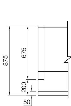
DETAIL A
