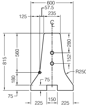
END VIEW DETAIL END A
