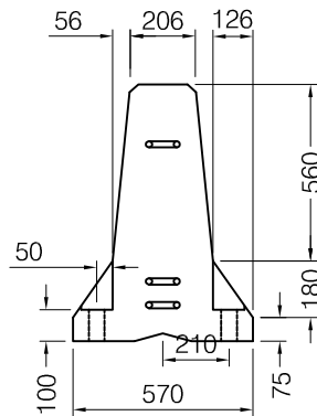
END VIEW DETAIL END A
