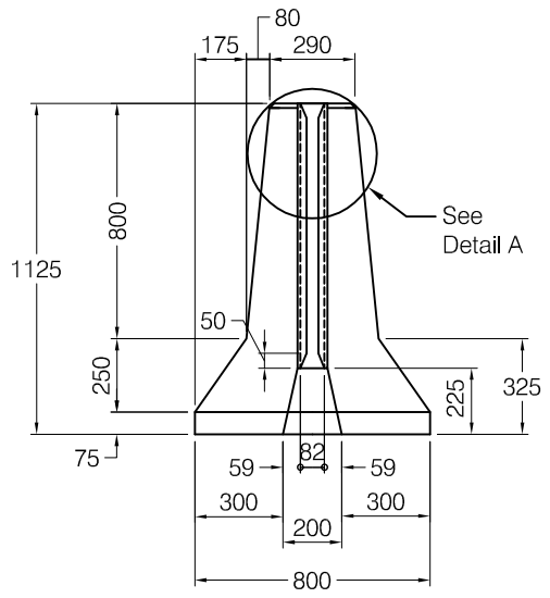
END VIEW DETAIL FEMALE CONNECTOR
